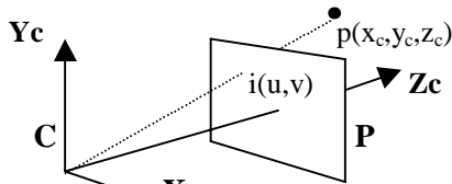
FIGURE 2. Camera model
