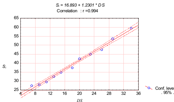
Figure 2. Correlation between the jaw's length and the diameter of the billet being captured.
