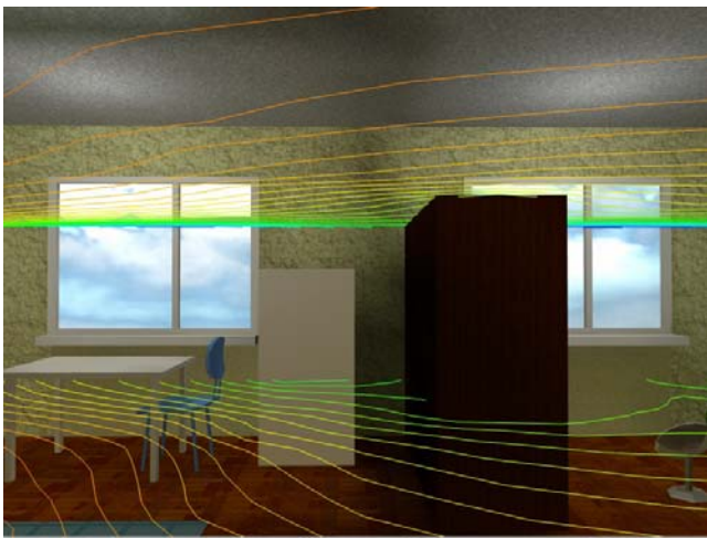
Figure 3: Temperature distribution on two section planes in a living room.
