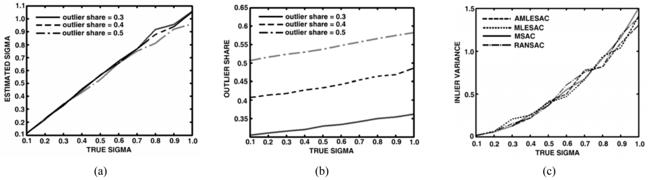
Figure 4 AMLESAC evaluation on line fitting problem (a) Estimated noise deviation \sigma of inliers plotted against true value. (b) Estimated outlier share 1 - \gamma plotted against noise deviation \sigma (c) Inlier variance \sigma^2 of 4 robust estimators for line fitting problem: RANSAC, MLESAC, MSAC, AMLESAC plotted against true deviation of inlier noise \sigma . Each value was calculated by averaging the results of 100 tests. (a) and (b) were computed for outlier shares 0.3, 0.4, 0.5. Comparison (c) is demonstrated for outlier share 0.5
