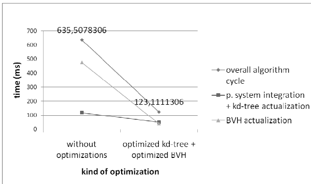
Figure 1: Time durations of the algorithm parts in 1000ms of simulation (98 particles).
