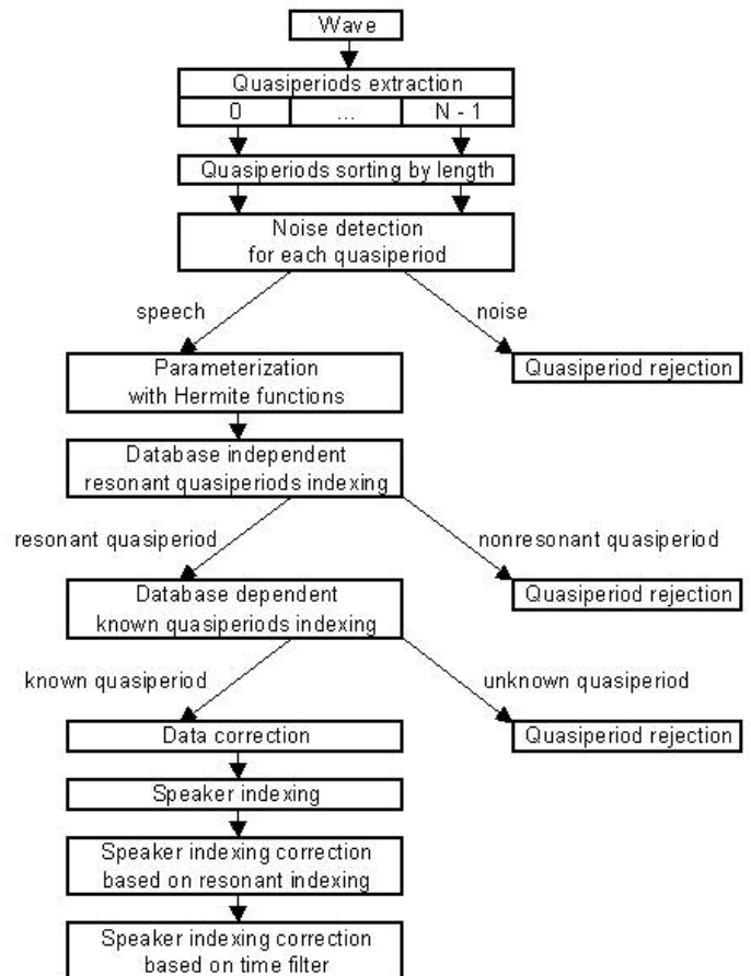
Figure 5: Scheme of indexing algorithm
