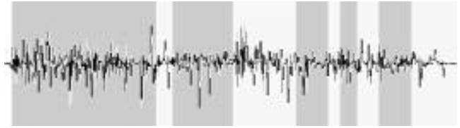
Figure 20: Indexed dialog based on Fourier expansion
