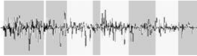
Figure 19: Indexed dialog based on Fourier expansion
