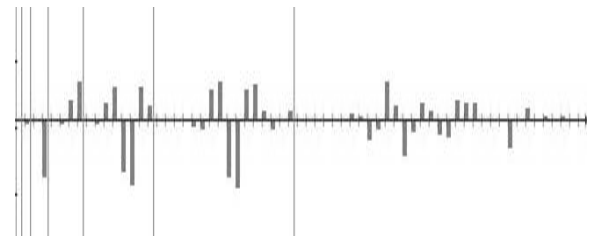
Figure 4: Hermite expansion coefficients for quasiperiod above
