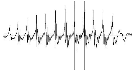
Figure 7: During each step we find the next border between quasiperiods.
