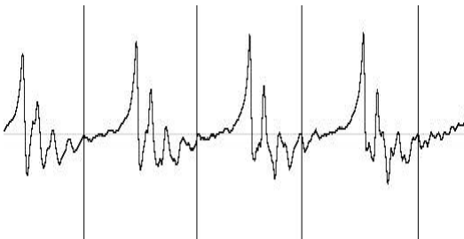
Figure 10: Quasiperiods detected by a modified algorithm.
