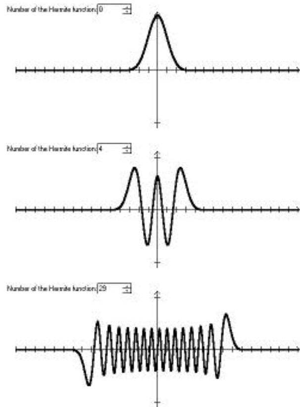
Figure 1: Hermite functions
