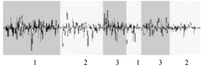
Figure 15: Original dialog (15sec, 3 speakers, 5 changes)
