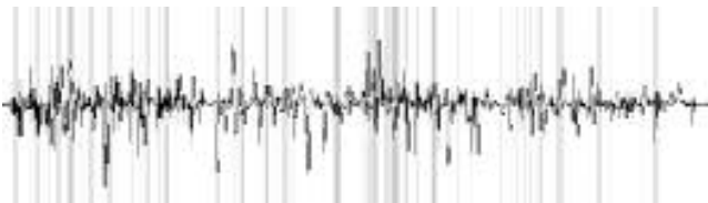
Figure 20: Indexed resonant quasiperiods
