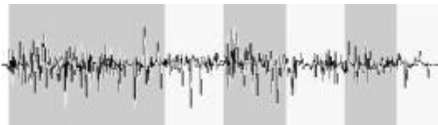
Figure 19: Indexed dialog based on Hermite expansion
