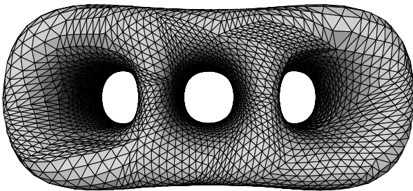
Figure 10: Remeshing of 3 holed torus using midpoint subdivision. The parameterization is smooth within each base domain triangle, but clearly not across base domain triangles.
