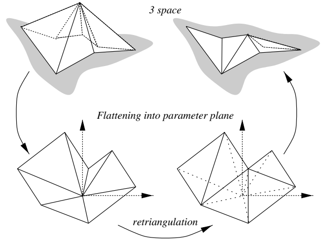
Figure 5: In order to remove a vertex p_i , its star (i) is mapped from 3-space to a plane using the map \mathcal{Z}^a . In the plane the central vertex is removed and the resulting hole retriangulated (bottom right).
