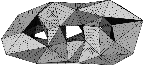
Figure 7: Base domain \varphi(|K^0|) . For each point p_i from the original mesh, its mapping \Pi(p_i) is shown with a dot on the base domain.
